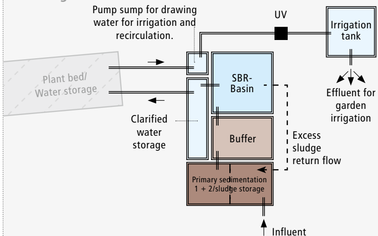
Plant diagram:
